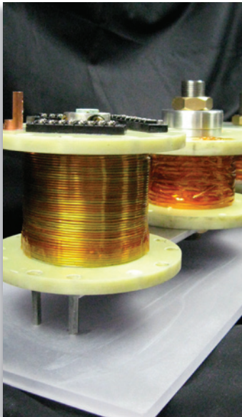
2009: A high field magnet coil fabricated by SuperPower with its 2G HTS wire and tested at NHMFL breaks another world record: magnetic field of 27.4 Tesla at 4.2K in 19.89 Tesla background field
